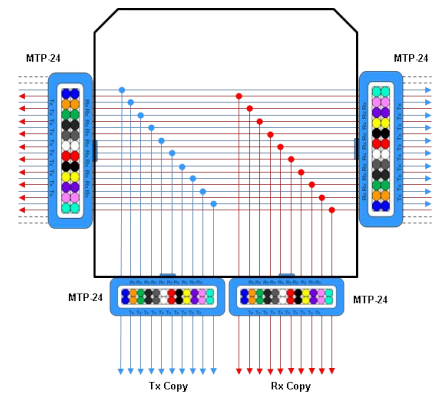
1/10 GIG SR-10 Assembly
