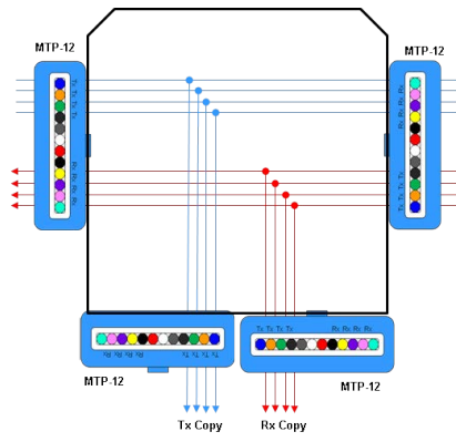
40 GIG SR-4 Assembly
