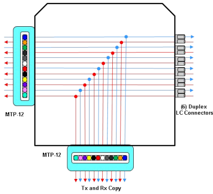
1/10 GIG Assembly
