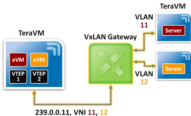
Figure 3: Multiple VTEP/VNI Scenario
